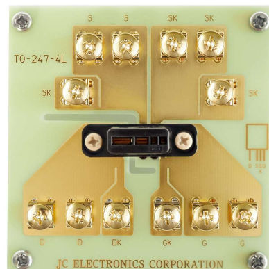
Test socket P/N : T4P-L214-ST-BK PC Board size : 85mm x 85mm PC Board thickness : 1.6mm
