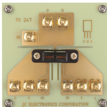
Test socket P/N : T3PH-L214-ST-BK PC Board size : 85mm x 85mm PC Board thickness : 1.6mm
